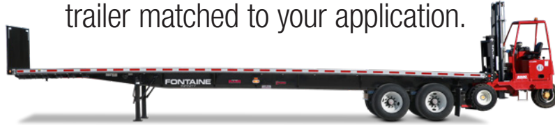
Infinity fixed or sliding tandem air ride forklift flatbed 45' or 48' configurations • Frame rating 80,000 lbs distributed Accommodates multiple forklift brands
